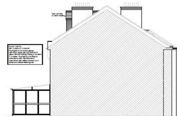
PROPOSED ADJ. SIDE ELEVATION (scale 1:50)
